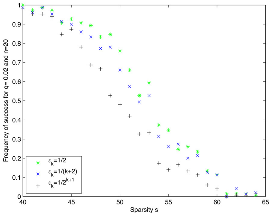
Fig. 3. Frequency of success vs. sparsity s.
