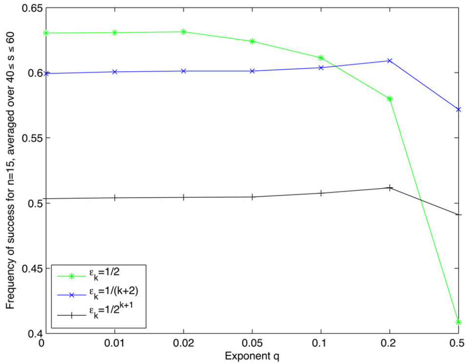
Fig. 2. Frequency of success vs. exponent q.
